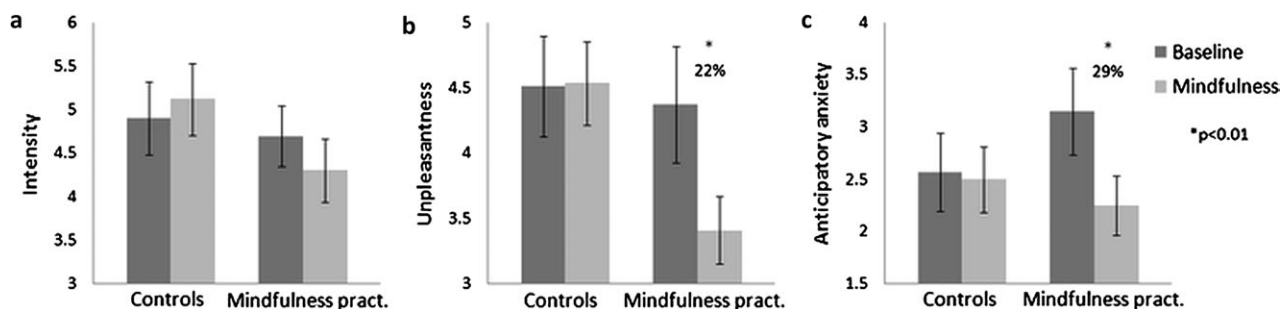
Figure 2. Pain (a) intensity, (b) unpleasantness, and (c) anticipatory anxiety ratings for mindfulness practitioners (pract.) and controls in the mindfulness and baseline condition. Error bars represent standard error of the mean.
