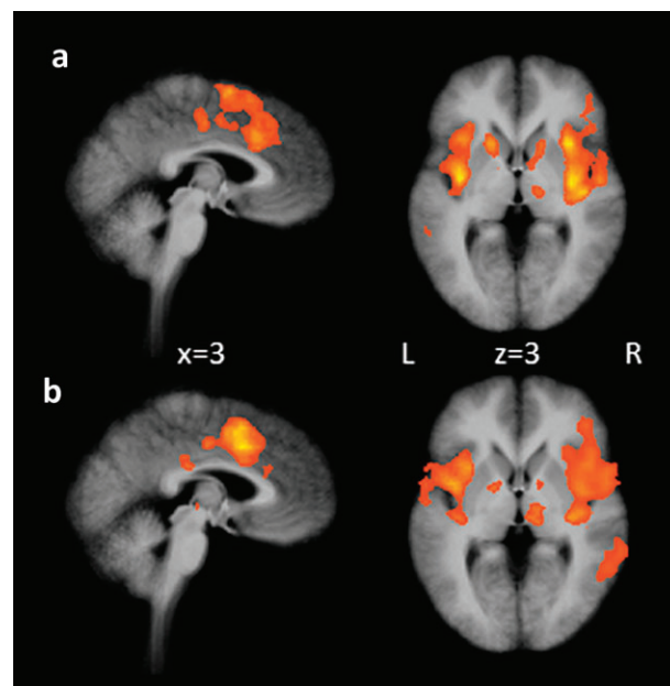
Figure 3. Activation in response to electric stimulation in (a) mindfulness practitioners and (b) controls during the baseline condition. Maps are the result of a whole-brain random effects analysis and are cluster level corrected for multiple comparisons at P < 0.05 (voxel threshold P < 0.001 , extent 6 for a and 7 for b).
